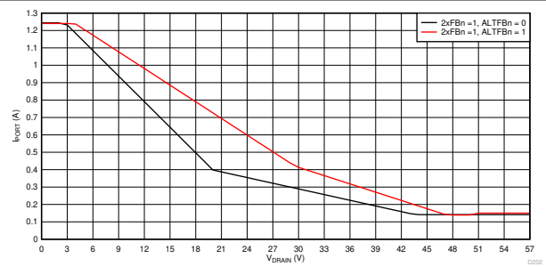
Figure 8-57. 2x Mode (2xFBn = 1) Foldback Curves, I_{PORT} vs V_{DRAIN}
