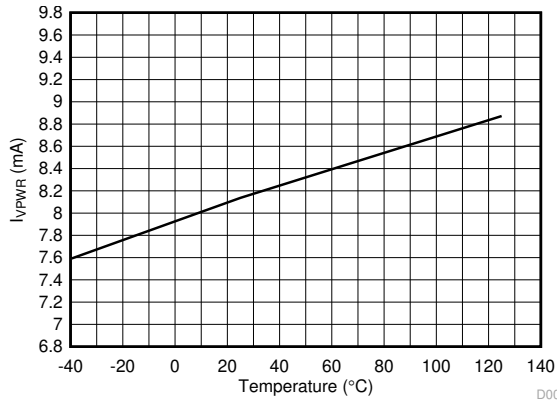
Figure 6-1. VPWR Current Consumption vs Temperature
