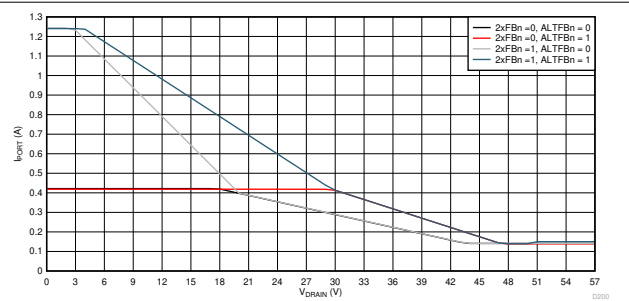
Figure 8-3. Foldback When the Port is Already ON: I_{LIM} vs V_{drain}
