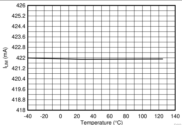
Figure 6-24. 1x Mode ( 2x\text{FBn} = 0 ) Current Limit vs Temperature
