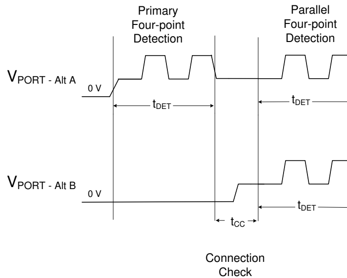
Figure 8-5. 4-Pair Port, Detection and Connection Check Waveforms with a Dual Signature Load
