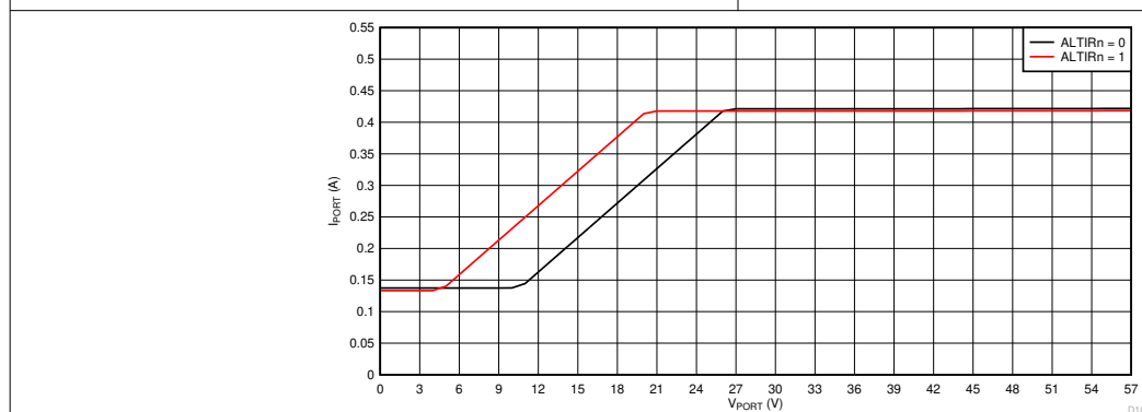
Figure 8-81. Inrush Foldback Curves, I PORT vs V PORT
