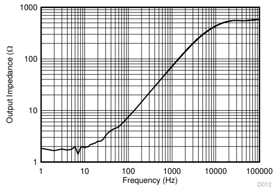
TMP23x-Q1: T_A = 25^\circ\text{C} , V_{DD} = 5\text{ V} , I_{OUT} = 100\ \mu\text{A} Figure 6-9. Output Impedance vs Frequency
