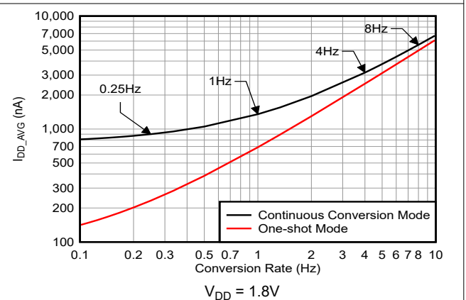
Figure 6-15. Average Quiescent Current vs Conversion Rate
