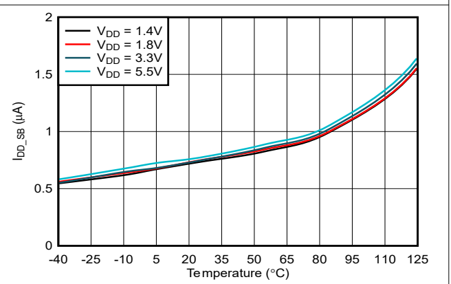
Figure 6-17. Standby Current vs Temperature
