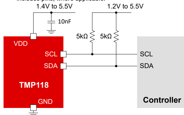
Figure 3-1. Simplified Schematic
