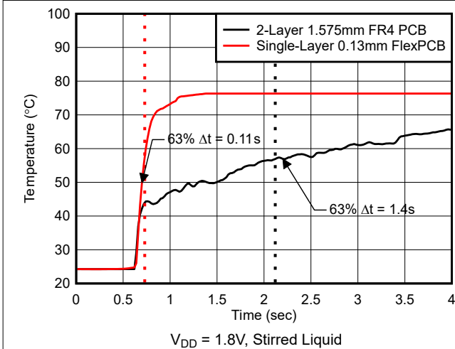
Figure 6-20. Temperature Measurement Response Time
