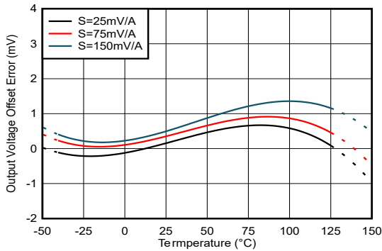
Figure 6-3. Offset Error vs Temperature: TMCS1133Bxx-Q1 Device Options
