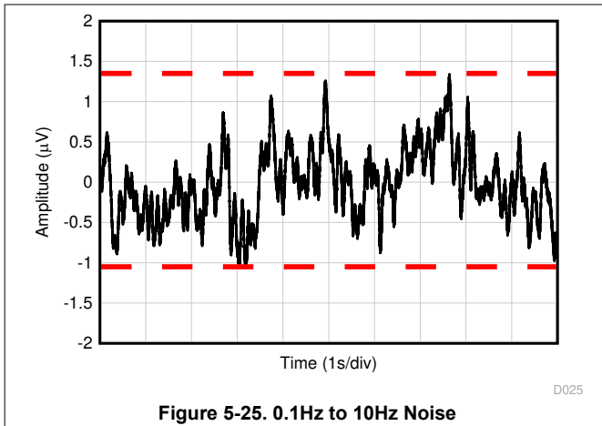
Figure 5-25. 0.1Hz to 10Hz Noise
