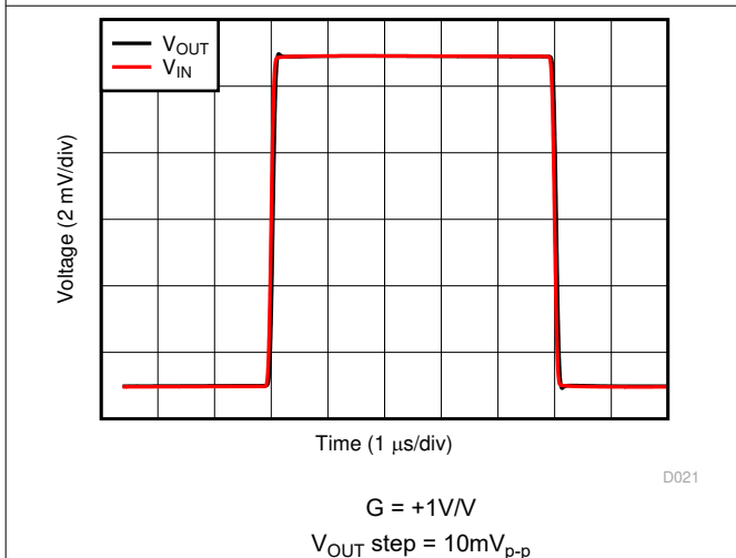
Figure 5-23. Small-Signal Step Response
