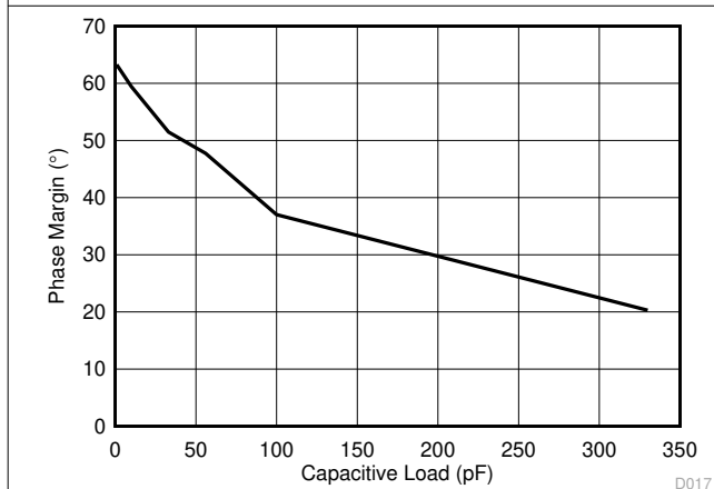
Figure 5-17. Phase Margin vs Capacitive Load
