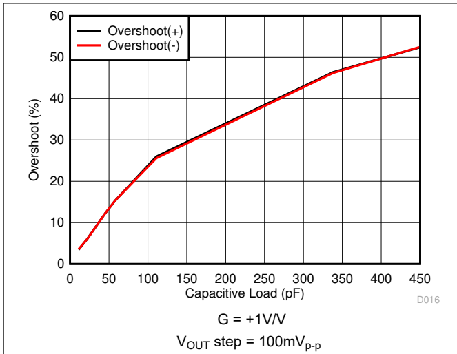
Figure 5-19. Small-Signal Overshoot vs Load Capacitance
