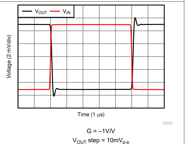
Figure 5-24. Small-Signal Step Response
