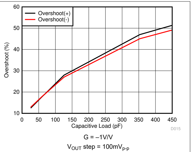
Figure 5-20. Small-Signal Overshoot vs Load Capacitance
