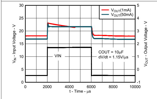
Figure 6-29. Line Transient Response for New Chip
