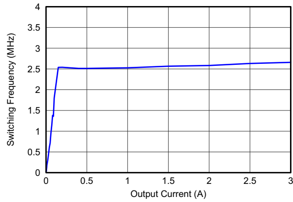
Figure 23. Switching Frequency
