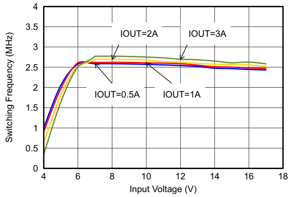
Figure 22. Switching Frequency
