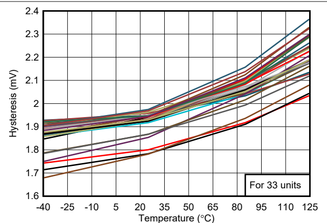
Figure 6-4. TLV3801 Hysteresis vs. Temperature
