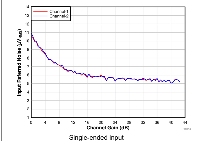
Figure 7-14. Input-Referred Noise vs Channel Gain
