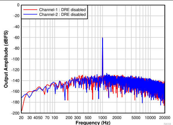
Figure 7-21. FFT With a -60\text{-dBr} Input With DRE Disabled
