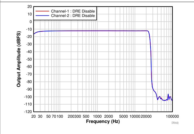
Figure 7-15. Frequency Response With a -12-dBr Input
