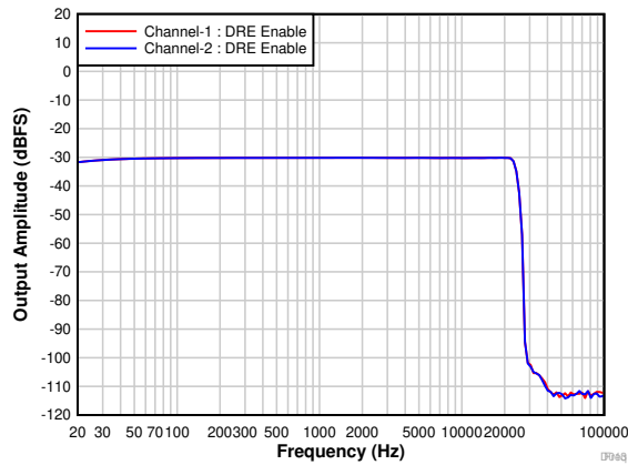
Figure 7-16. Frequency Response With a -30\text{-dBr} Input
