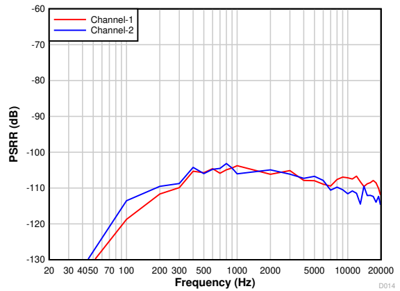
Figure 7-17. Power-Supply Rejection Ratio vs Ripple Frequency With 100\text{-mV}_{pp} Amplitude
