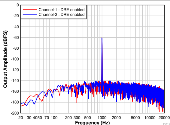
Figure 7-20. FFT With a -60\text{-dBr} Input With DRE Enabled
