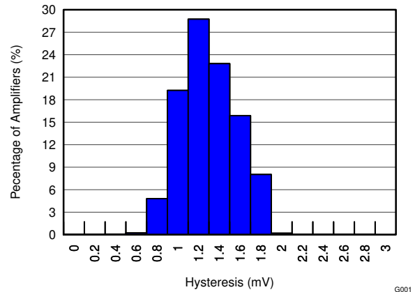
Figure 6-2. Hysteresis Distribution
