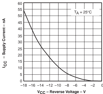
SUPPLY CURRENT VS REVERSE VOLTAGE
