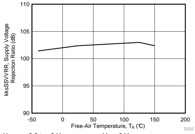
Figure 29. Supply-Voltage Rejection Ratio vs Free-Air Temperature
