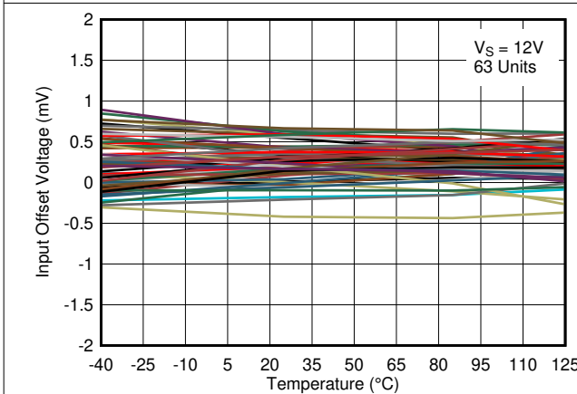
Figure 6-20. Input Offset Voltage vs. Temperature at 12V
