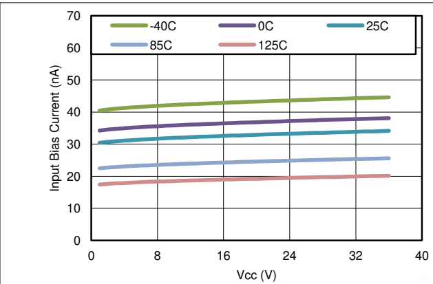
Figure 6-2. Input Bias Current vs Supply Voltage
