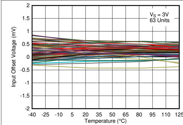
Figure 6-18. Input Offset Voltage vs. Temperature at 3V
