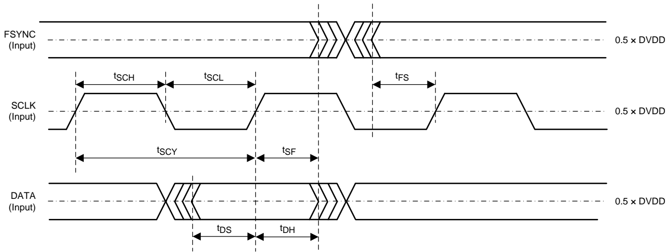
Figure 36. Serial Audio Timing
