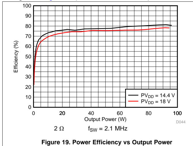
Figure 19. Power Efficiency vs Output Power
