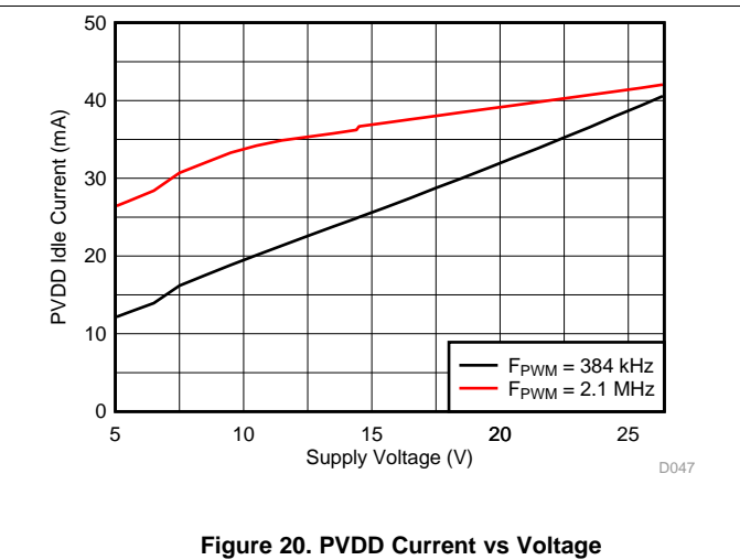
Figure 20. PVDD Current vs Voltage
