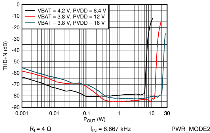
Figure 6-9. THDN vs Output Power
