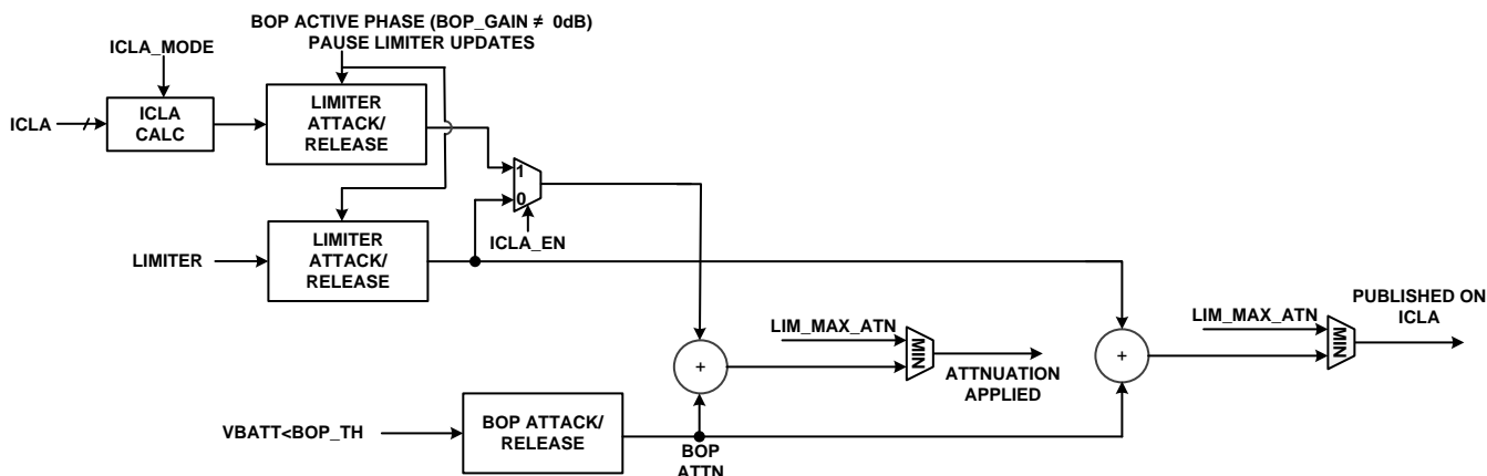
Figure 59. Limiter and Brown Out Prevention Interaction Diagram
