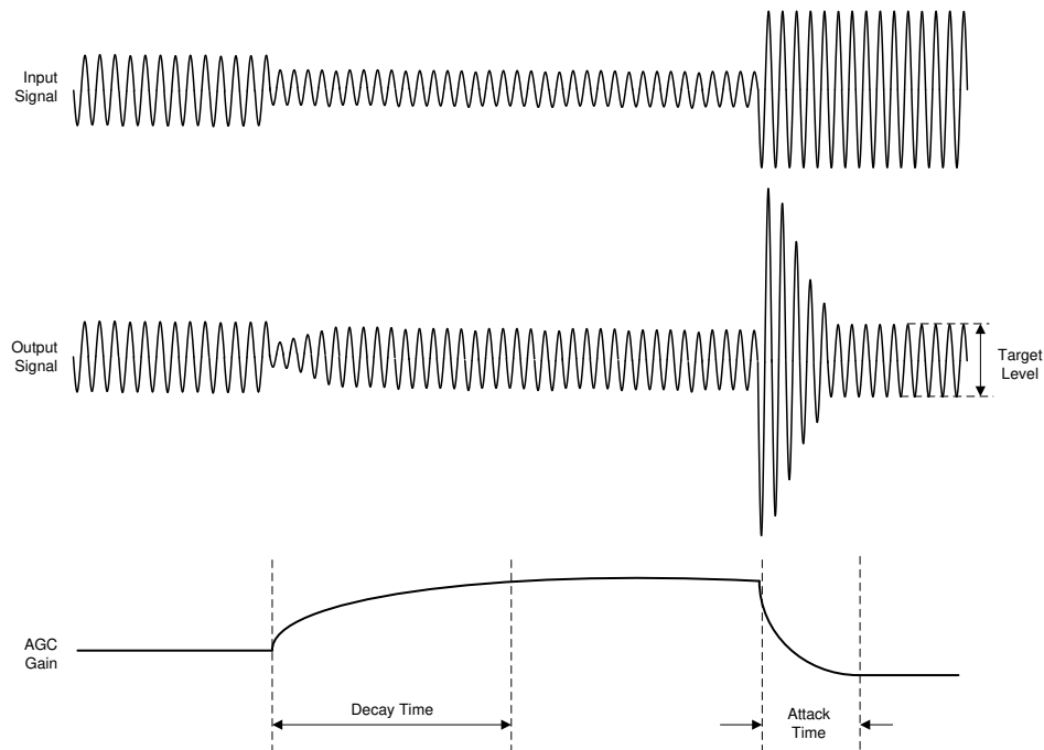
Figure 6-101. AGC Characteristics
