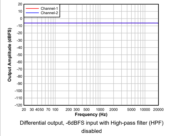
Figure 5-18. DAC Frequency Response
