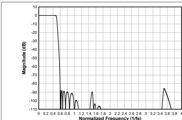
Figure 7-54. Low-latency Decimation Filter Magnitude Response
