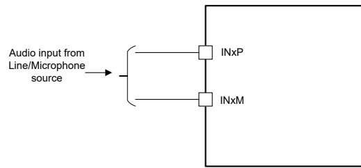
Figure 7-16. Differential DC-Coupled Input Connection (ADC_CHx_INSRC set to 2'b00 and ADC_CHx_CM_TOL set to 2'b01 or 2'10)
