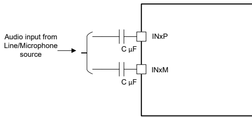
Figure 7-15. Differential AC-Coupled Input Connection (ADC_CHx_INSRC set to 2'b00 and ADC_CHx_CM_TOL set to 2'b00 or 2'b01 or 2'10)
