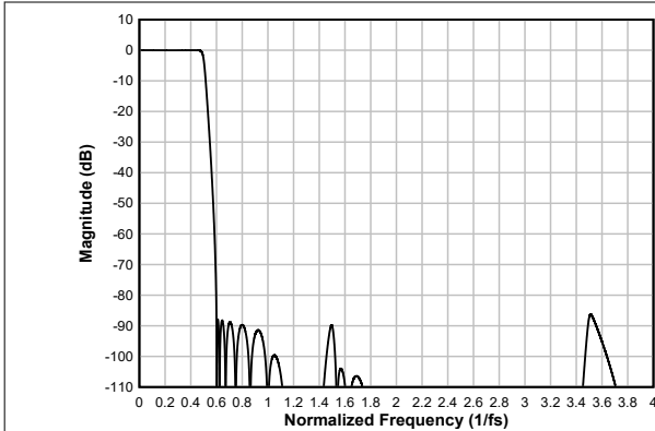
Figure 7-52. Low-latency Decimation Filter Magnitude Response
