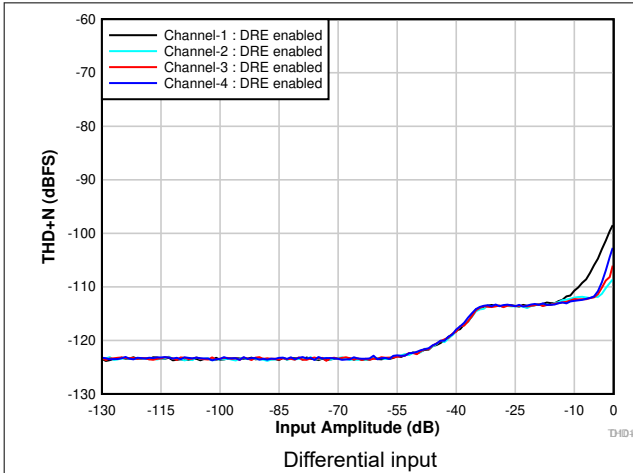
Figure 6-5. THD+N vs Input Amplitude With DRE Enabled
