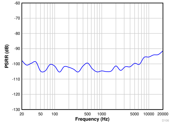
Figure 6-16. Power-Supply Rejection Ratio With Ripple Frequency With 100-mV pp Amplitude
