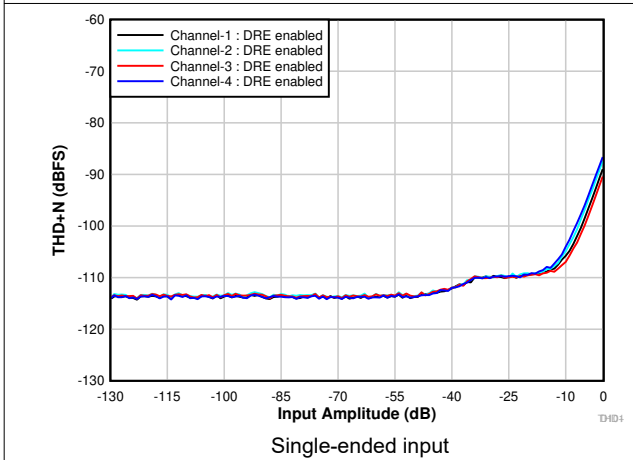
Figure 6-7. THD+N vs Input Amplitude With DRE Enabled
