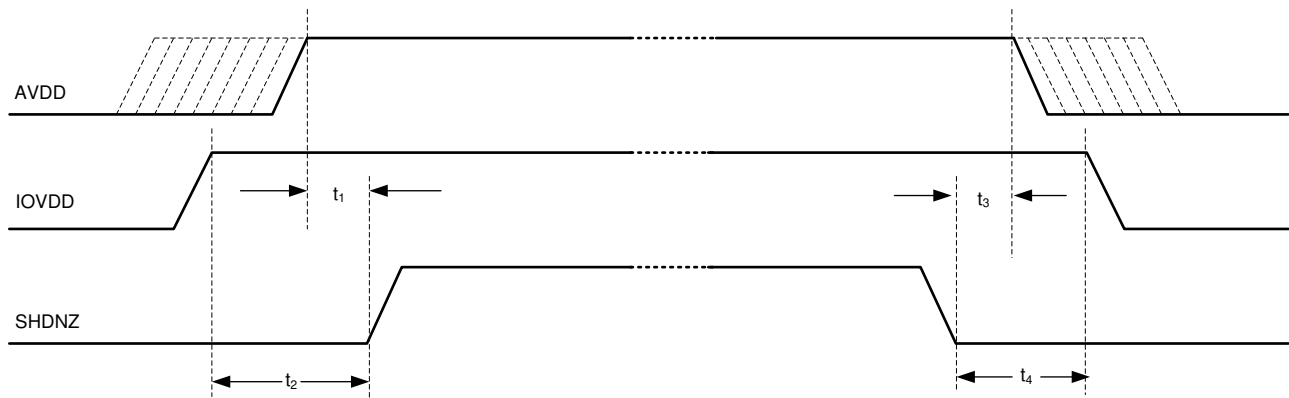
Figure 9-7. Power-Supply Sequencing Requirement Timing Diagram
