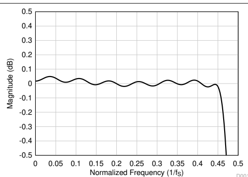
Figure 7-20. Linear Phase Decimation Filter Pass-Band Ripple
