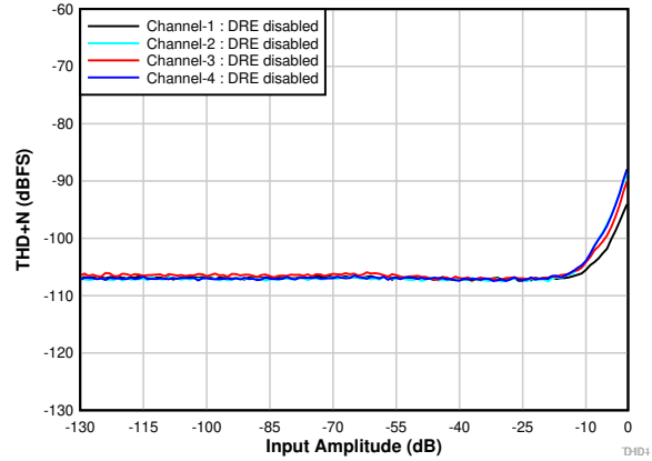
Differential input with AVDD = 1.8 V and VREF = 1.375 V
