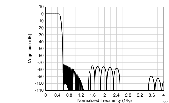
Figure 7-19. Linear Phase Decimation Filter Magnitude Response
