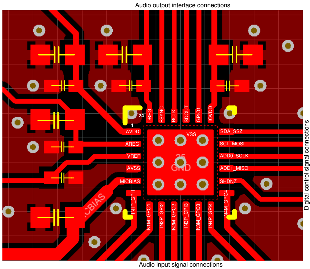
Figure 9-8. Layout Example
