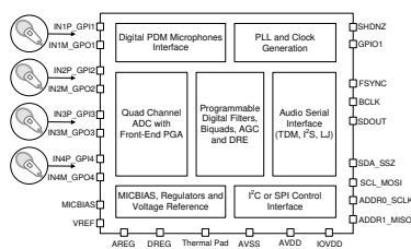
Simplified Block Diagram
