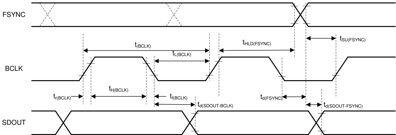
Figure 6-3. TDM (With BCLK_POL = 1), I 2 S, and LJ Interface Timing Diagram
