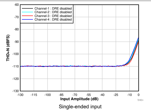
Figure 6-8. THD+N vs Input Amplitude With DRE Disabled
