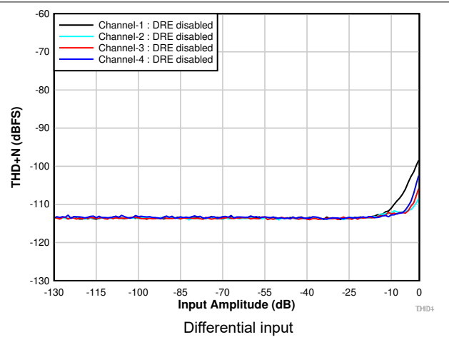
Figure 6-6. THD+N vs Input Amplitude With DRE Disabled
