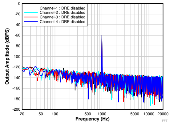
Figure 6-20. FFT With a -60-dBr Input With DRE Disabled
