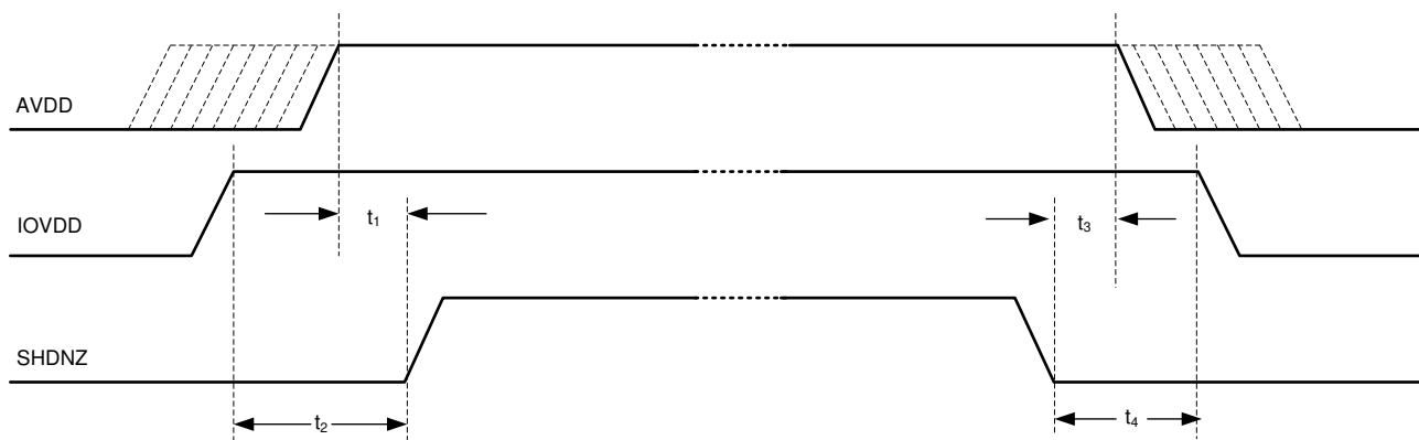
Figure 8-7. Power-Supply Sequencing Requirement Timing Diagram
