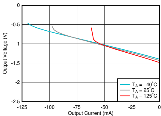
Output slammed to the negative rail
