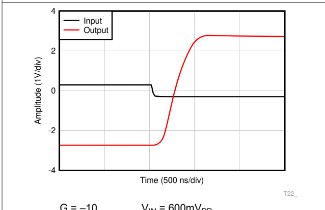
G = -10 V_{IN} = 600\text{mV}_{PP} Figure 6-57. Overload Recovery
