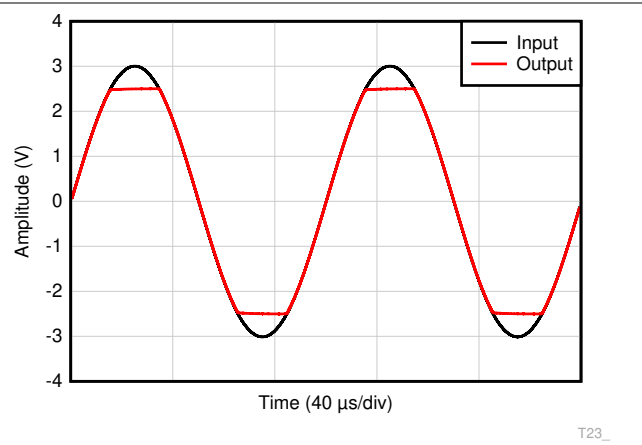
G = 1 V_{IN} = 6\text{V}_{PP} Figure 6-56. No Phase Reversal
