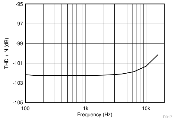
Figure 7-18. THD + N vs Frequency V_S = 5.5\text{ V} V_{ICM} = 2.5\text{ V} R_L = 10\text{ k}\Omega Gain = 1 BW = 80 kHz V_{OUT} = 0.5\text{ V}_{rms}
