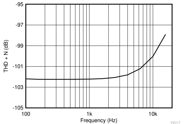
Figure 7-17. THD + N vs Frequency V_S = 5.5\text{ V} V_{ICM} = 2.5\text{ V} R_L = 2\text{ k}\Omega Gain = 1 BW = 80 kHz V_{OUT} = 0.5\text{ V}_{rms}
