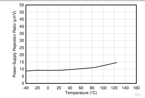
Figure 6-26. DC PSRR vs Temperature
