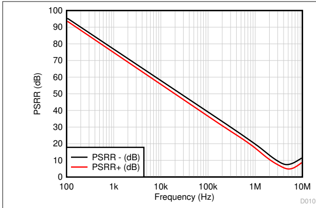
Figure 6-25. PSRR vs Frequency
