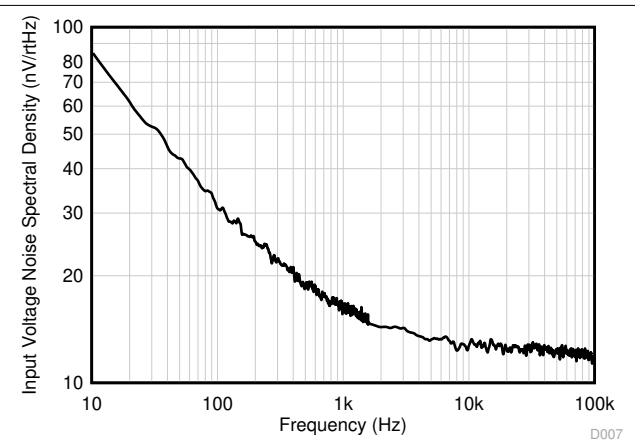
Figure 6-30. Input Voltage Noise Spectral Density
