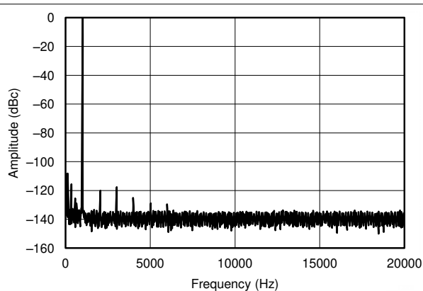
Figure 9-5. Output Spectrum of a 1-mW, 1-kHz Tone into a 32- \Omega Load
