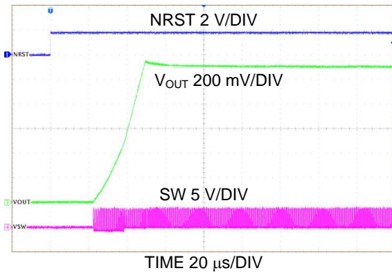
Figure 45. Start-up with NRST, Forced PWM
