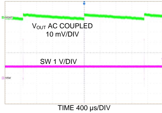
Figure 43. Output Voltage Ripple, PFM Mode
