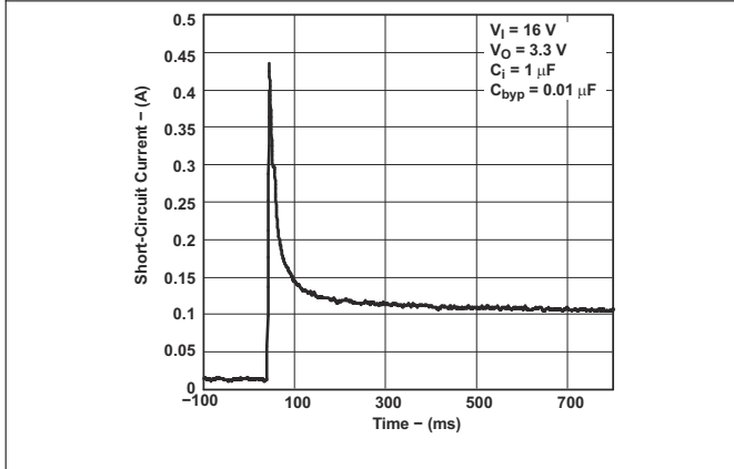
Figure 6-11. Short-Circuit Current vs Time for Legacy Chip
