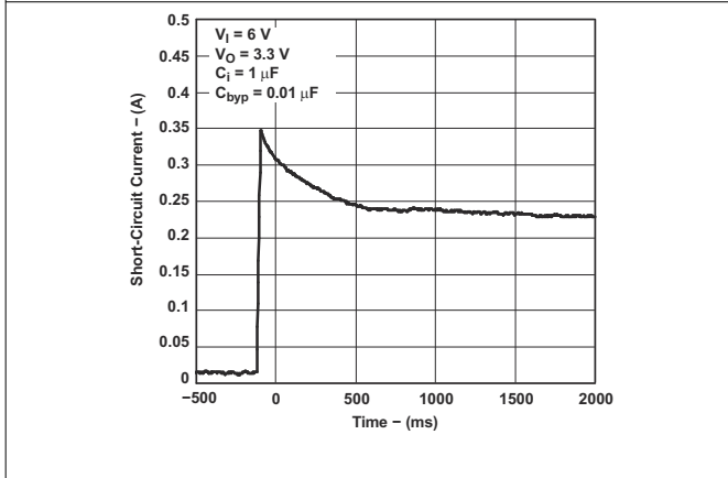
Figure 6-9. Short-Circuit Current vs Time for Legacy Chip
