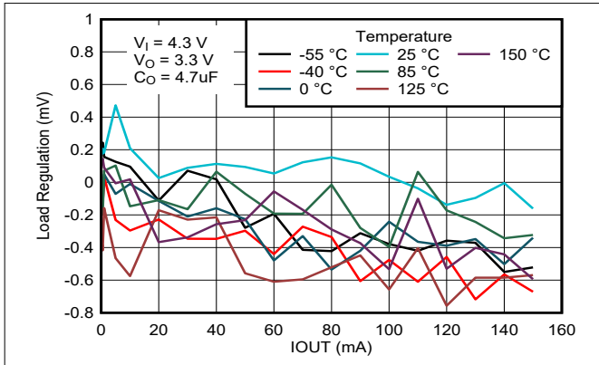
Figure 6-7. Output Regulation vs Load Current for New Chip
