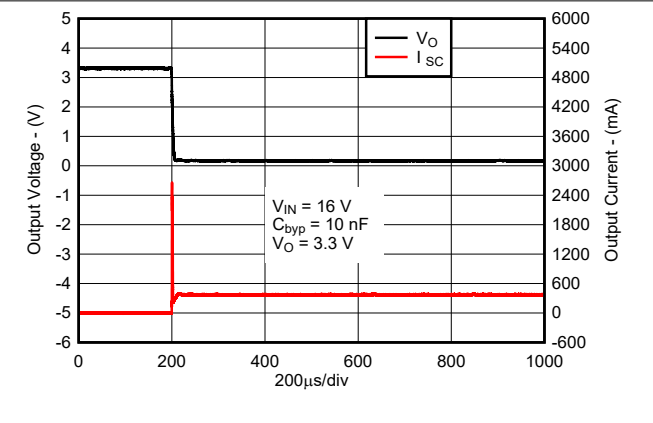
Figure 6-12. Short-Circuit Current vs Time for New Chip
