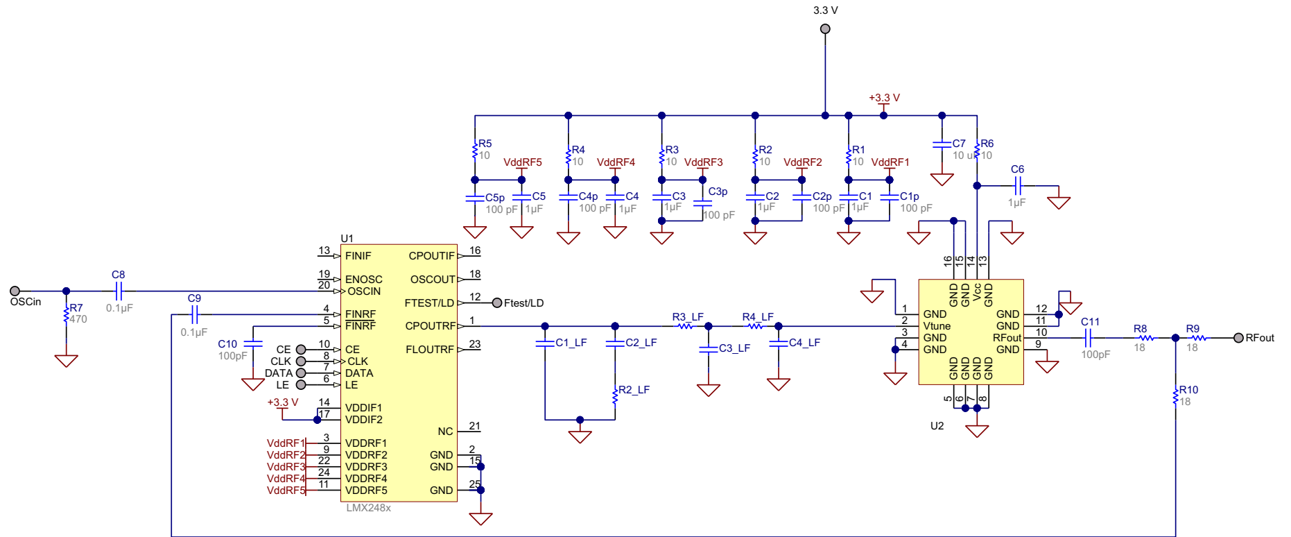
Figure 24. Typical Application
