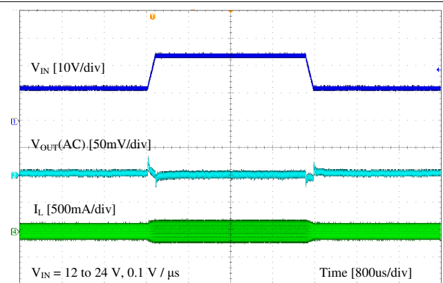
Figure 8-8. Line Transient
