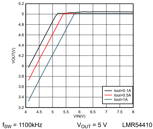
Figure 6-9. 5-V Dropout
