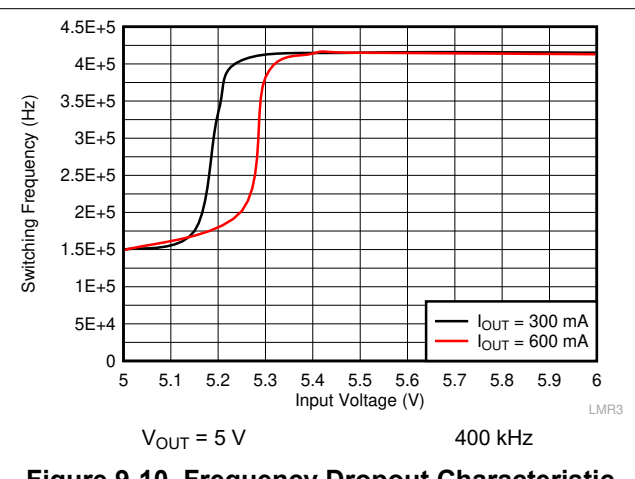
Figure 9-10. Frequency Dropout Characteristic
