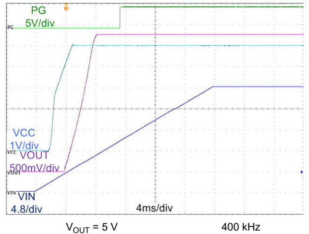
Figure 9-14. Start-Up Waveform
