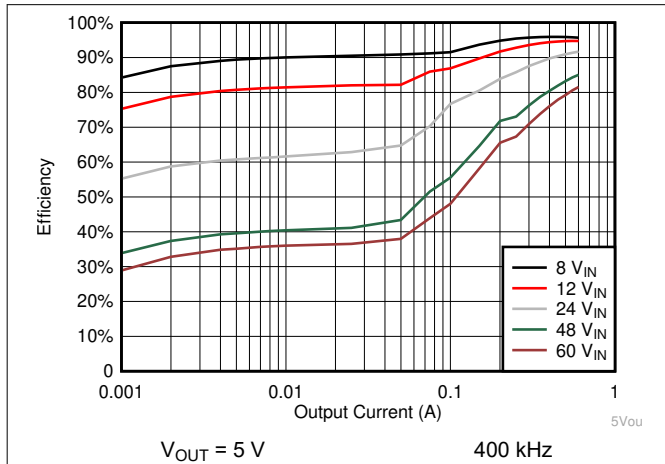
Figure 9-5. Efficiency
