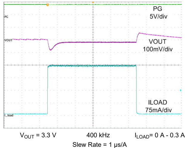
Figure 9-16. Load Transient
