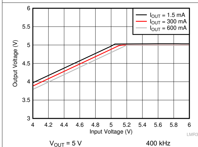
Figure 9-9. Overall Dropout Characteristic
