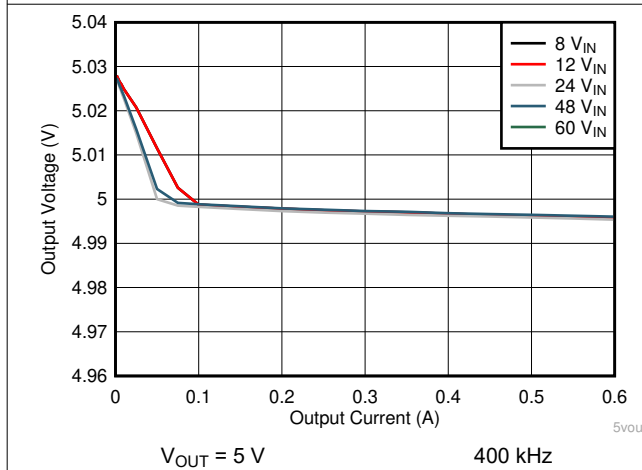
Figure 9-7. Load Regulation
