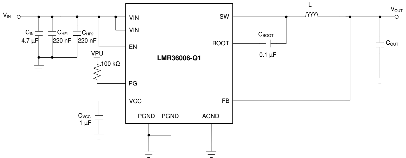
Figure 9-2. Example Applications Circuit (Fixed 3.3 V Output)
