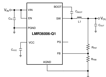
Simplified Schematic
