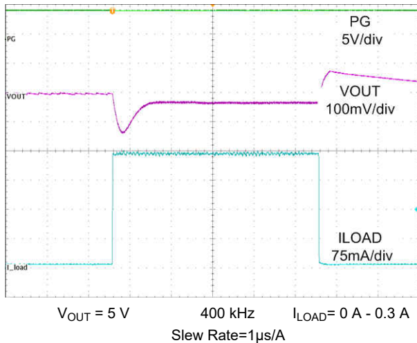
Figure 9-15. Load Transient
