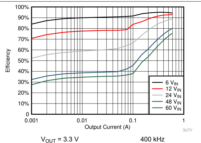
Figure 9-6. Efficiency
