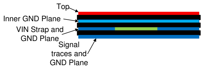
Figure 11-2. Example Layout
