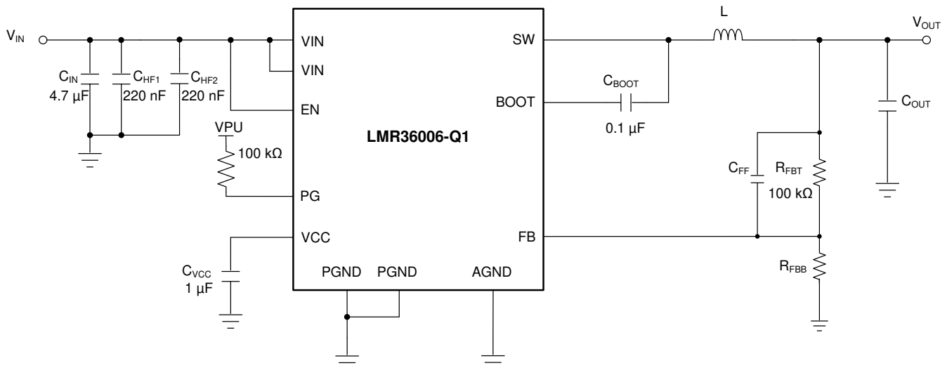
Figure 9-1. Example Applications Circuit (Adjustable Output)
