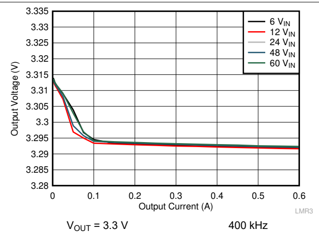
Figure 9-8. Load Regulation
