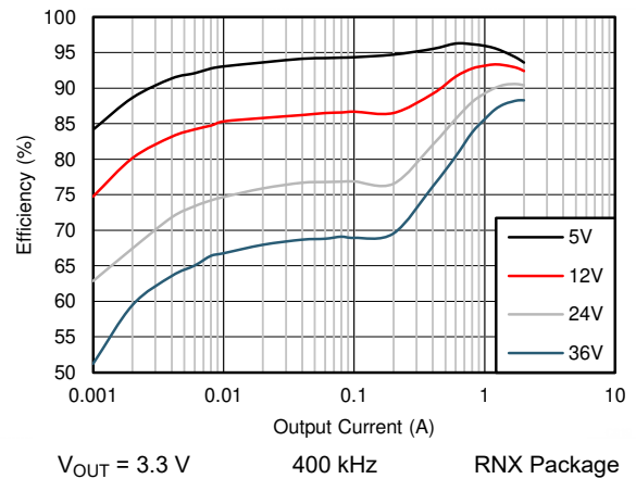
Figure 8-12. Efficiency
