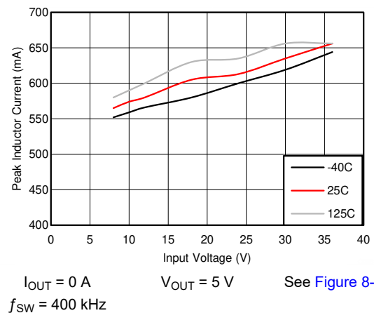
Figure 6-6. I_{PEAK-MIN}
