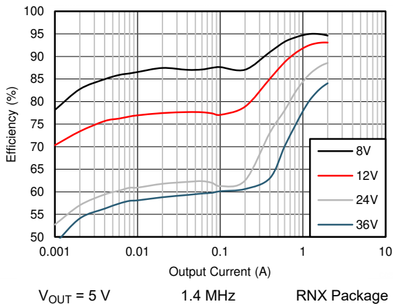
Figure 8-13. Efficiency
