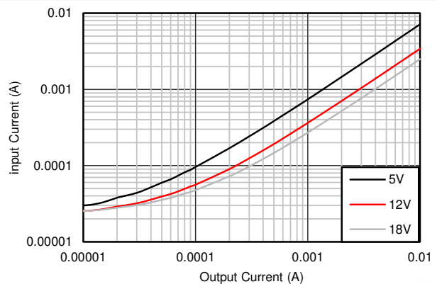
Figure 8-5. Input Supply Current vs Output Current for 3.3-V Fixed Output Option
