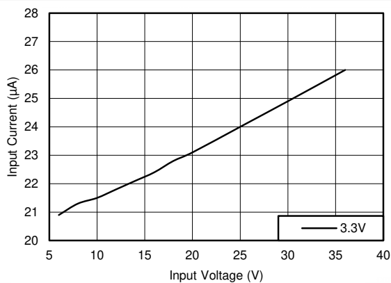
Figure 8-4. No-load Input Supply Current for 3.3-V Fixed Output Option
