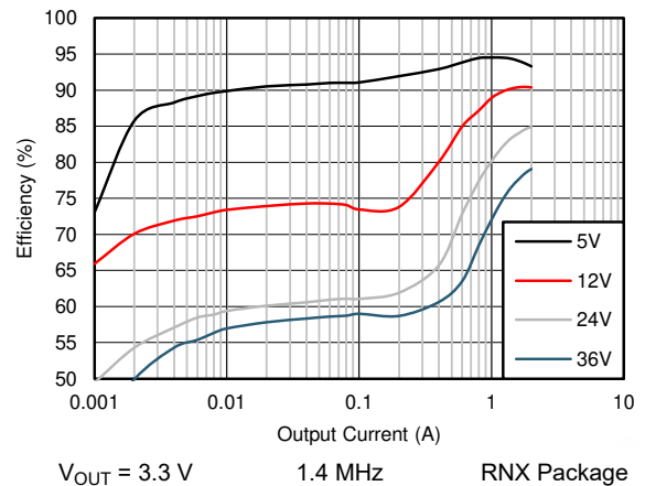
Figure 8-14. Efficiency
