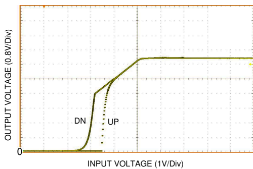
Figure 6-5. UVLO Thresholds
