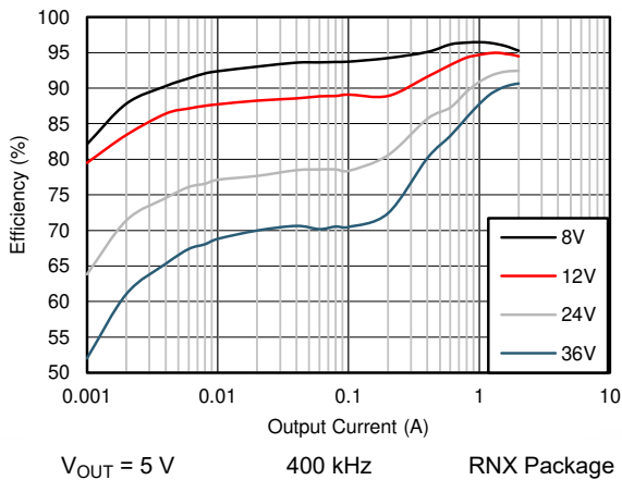
Figure 8-11. Efficiency
