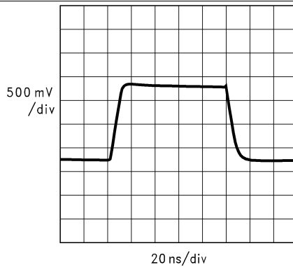
Figure 33. Large Signal Pulse Response, Av = -1, VS = ±15 V
