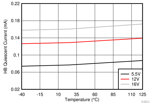
Figure 6-3. HB Quiescent Current
