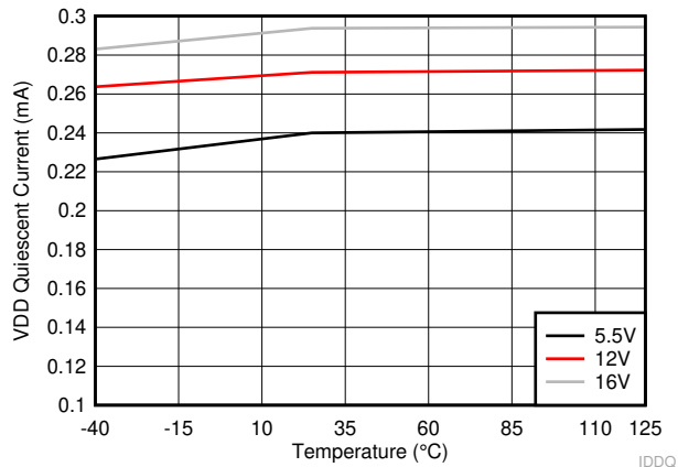
Figure 6-2. VDD Quiescent Current
