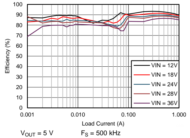
Figure 60. Efficiency
