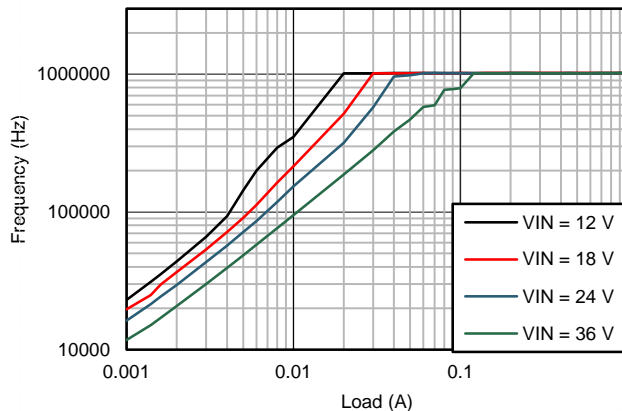
Figure 34. Switching Frequency Decreases With Lower Load Current in PFM Operation V OUT = 5 V, F S = 1 MHz
