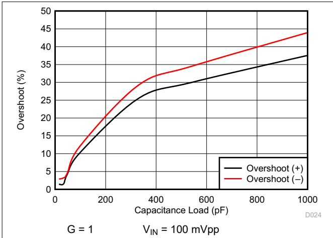
Figure 6-18. Small Signal Overshoot vs Capacitive Load
