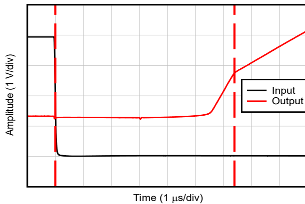
Time (1 \mu\text{s}/\text{div} ) G = -10
