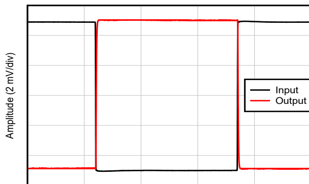
Time (20 \mu\text{s}/\text{div} ) G = -1 , R_L = \text{open} , R_{FB} = 10\text{K} See Section 6
