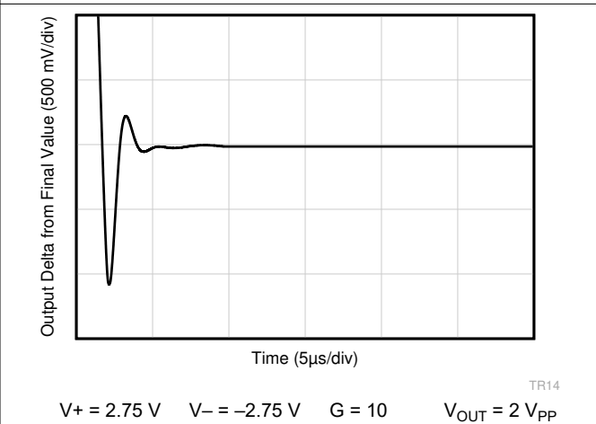
Figure 6-48. Large Signal Settling Time (Falling Edge)
