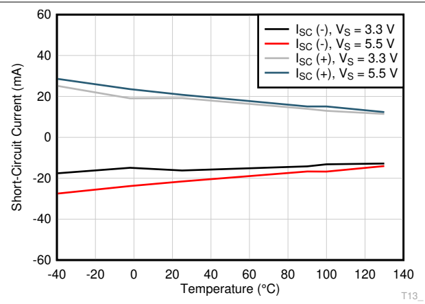
Figure 6-20. Short Circuit Current vs Temperature
