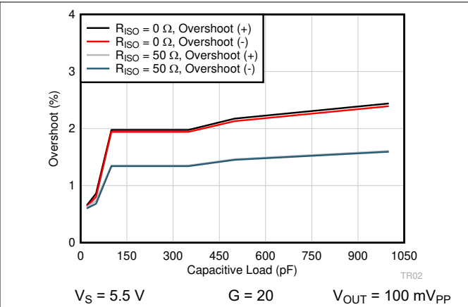
Figure 6-44. Small-Signal Overshoot vs Capacitive Load
