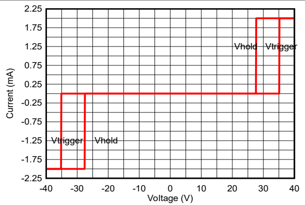
Figure 5-4. DC-IV Curve
