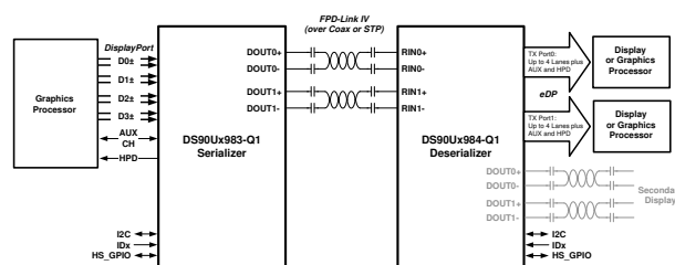
Simplified Application Diagram
