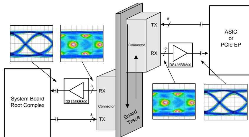
Figure 9. Typical Application
