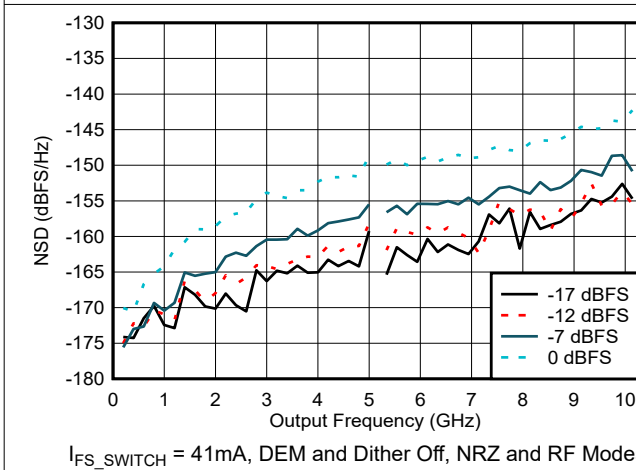
Figure 6-66. NSD vs Output Frequency and Digital Amplitude
