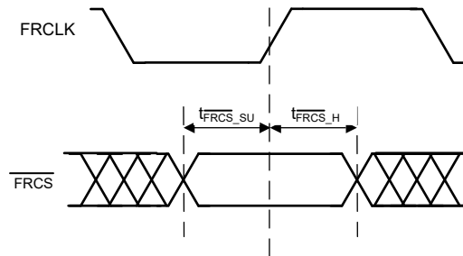
Figure 6-7. FRCS Timing Diagram
