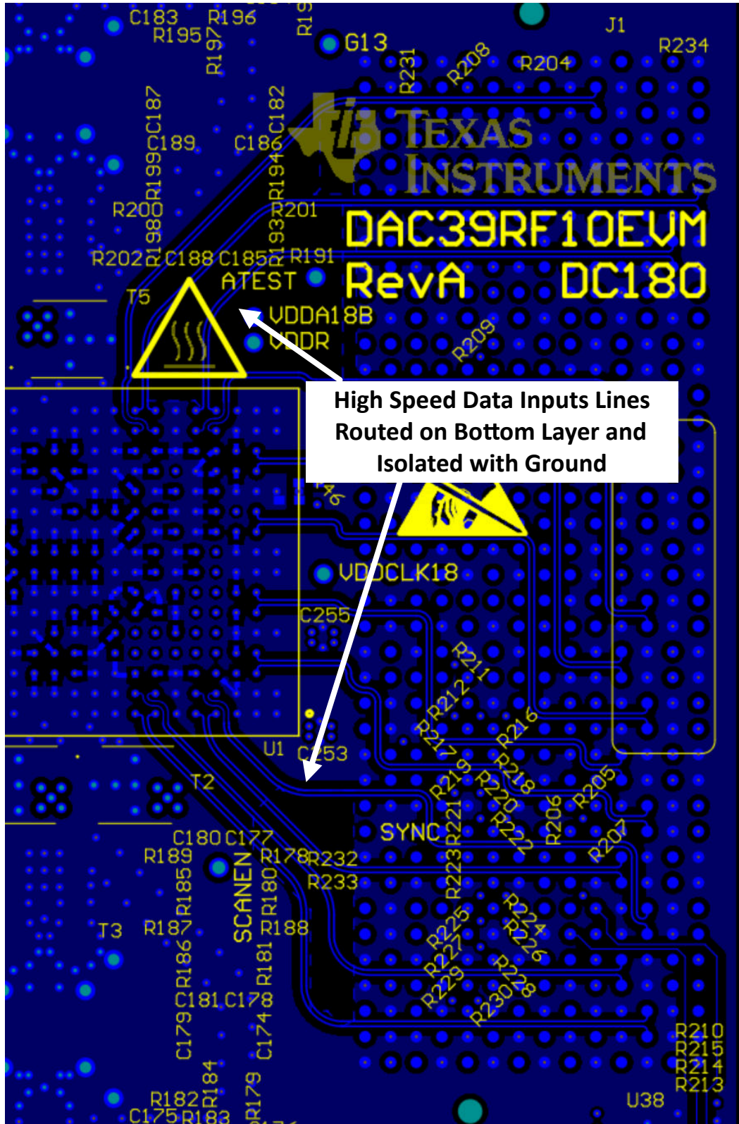
Figure 8-30. Serdes Bottom Layer Routing with Ground Isolation
