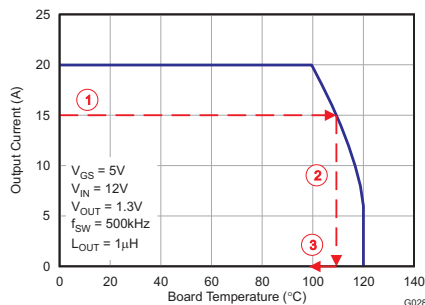
Figure 33. Power Block SOA
