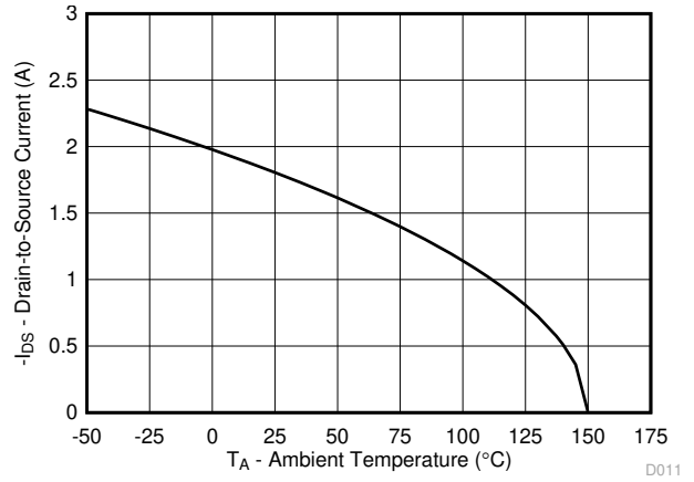
Figure 5-11. Maximum Drain Current vs Temperature
