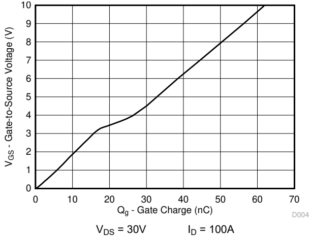
Figure 4-4. Gate Charge
