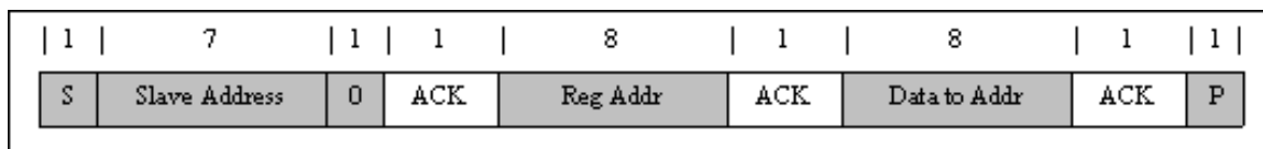
Figure 29. Single Write
