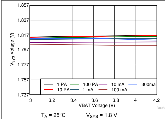
Figure 10-22. 1.8 V sys Line Regulation
