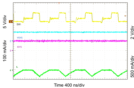
Figure 10-28. Light Load Operation Showing SW
