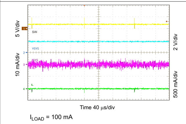
Figure 10-27. Light Load Operation Showing SW
