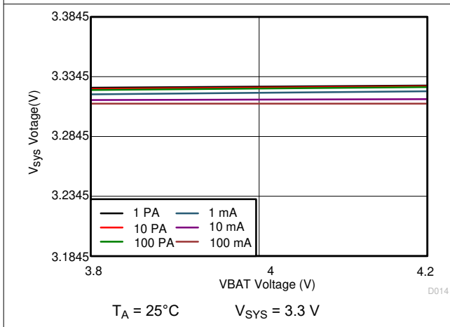
Figure 10-24. 3.3 V sys Line Regulation
