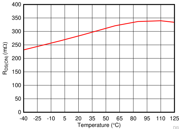
Figure 8-13. R_{DS(ON)} of Low Side MOSFET vs Temperature
