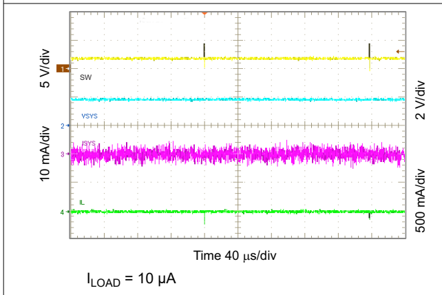
Figure 10-26. Light Load Operation Showing SW
