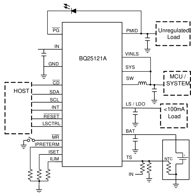
Simplified Schematic
