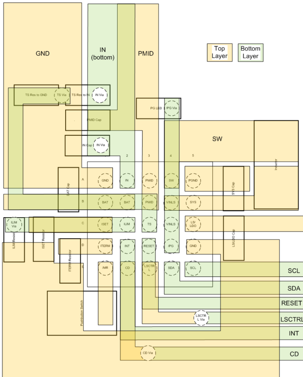
Figure 12-1. BQ25121A Layout
