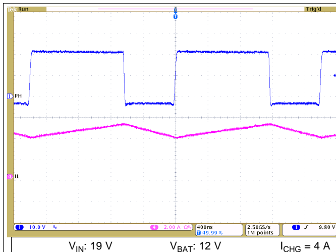
Figure 21. Continuous Conduction Mode Switching Waveform
