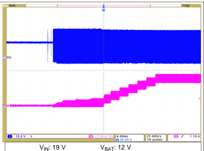
Figure 22. Battery Charging Soft Start
