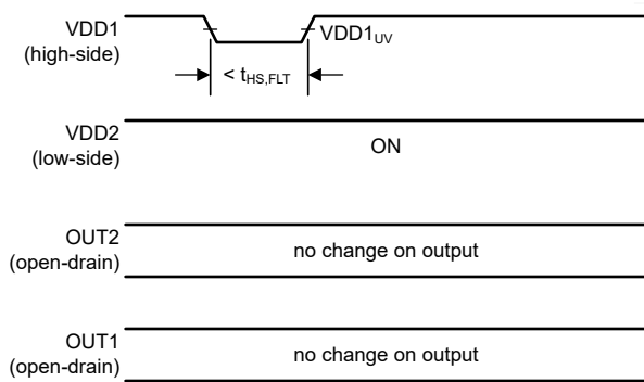
Figure 6-11. Output Response to a Short Brownout Event on VDD1
