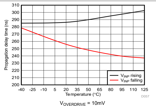
Figure 5-53. Cmp0 Propagation Delay vs Temperature
