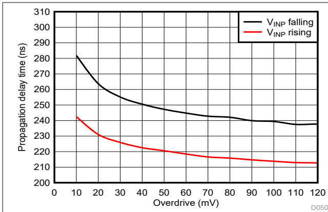
Figure 5-54. Cmp1 Propagation Delay vs Overdrive
