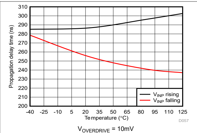
Figure 5-37. Cmp0 Propagation Delay vs Temperature
