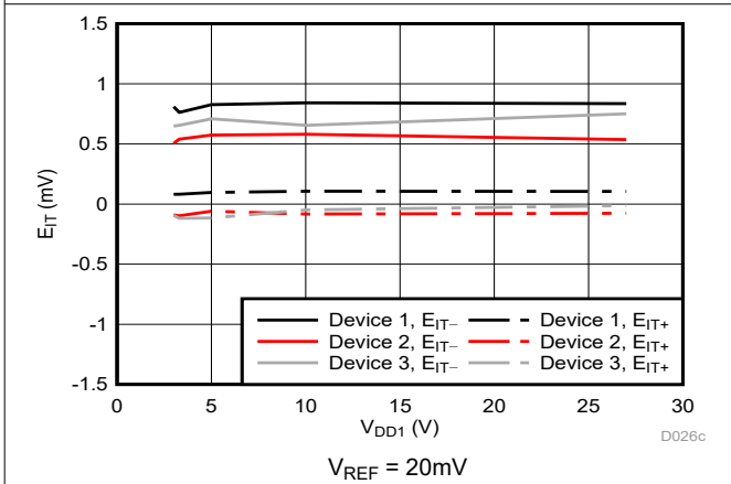
Figure 5-26. Cmp1 Trip Threshold Error vs Supply Voltage
