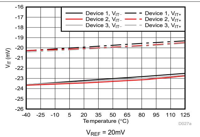
Figure 5-25. Cmp1 Trip Threshold vs Temperature
