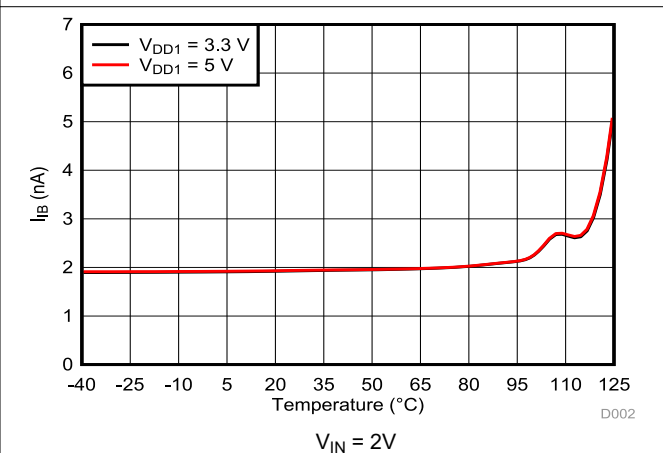
Figure 5-41. Input Bias Current vs Temperature
