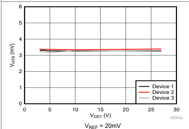
Figure 5-28. Cmp1 Trip Threshold Hysteresis vs Supply Voltage
