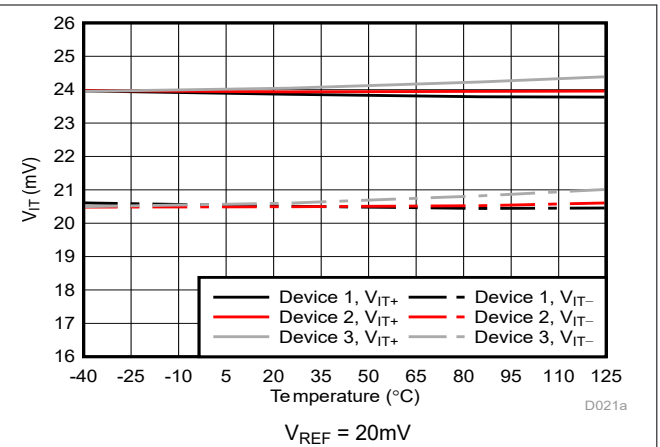
Figure 5-7. Cmp0 Trip Threshold vs Temperature
