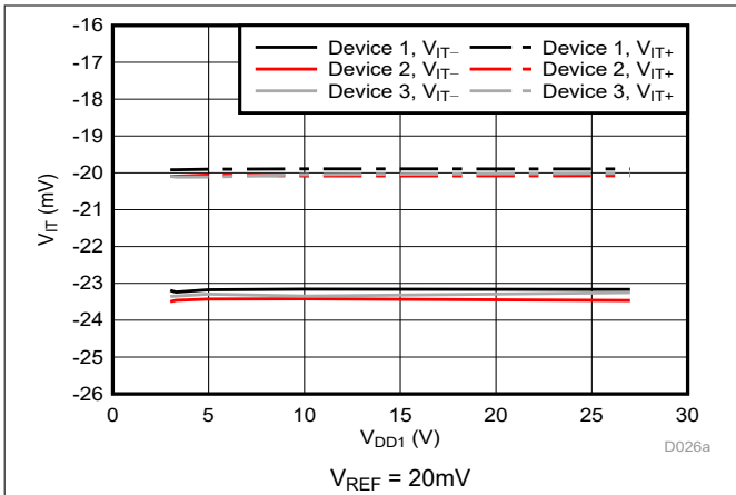
Figure 5-24. Cmp1 Trip Threshold vs Supply Voltage
