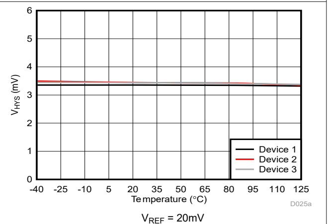
Figure 5-11. Cmp0 Trip Threshold Hysteresis vs Temperature
